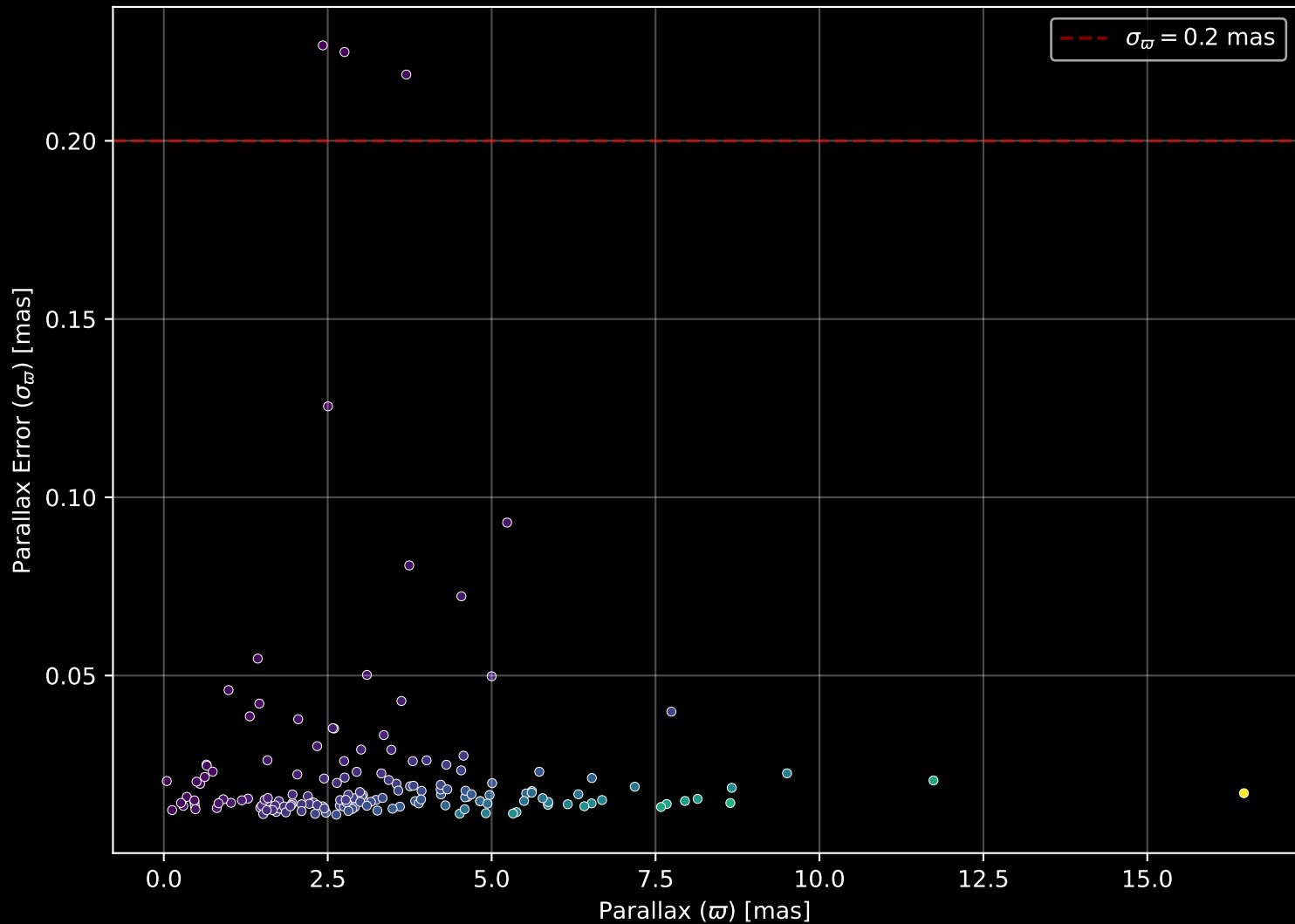
APOGEE DR17 Field: [041+53_MGA] Parallax Quality (n= 161)
