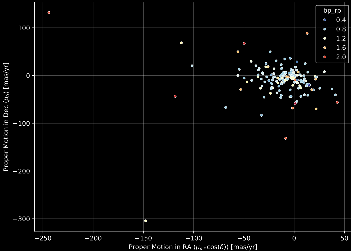
APOGEE DR17 Field: [041+53_MGA] Proper Motion Diagram (n= 161)
