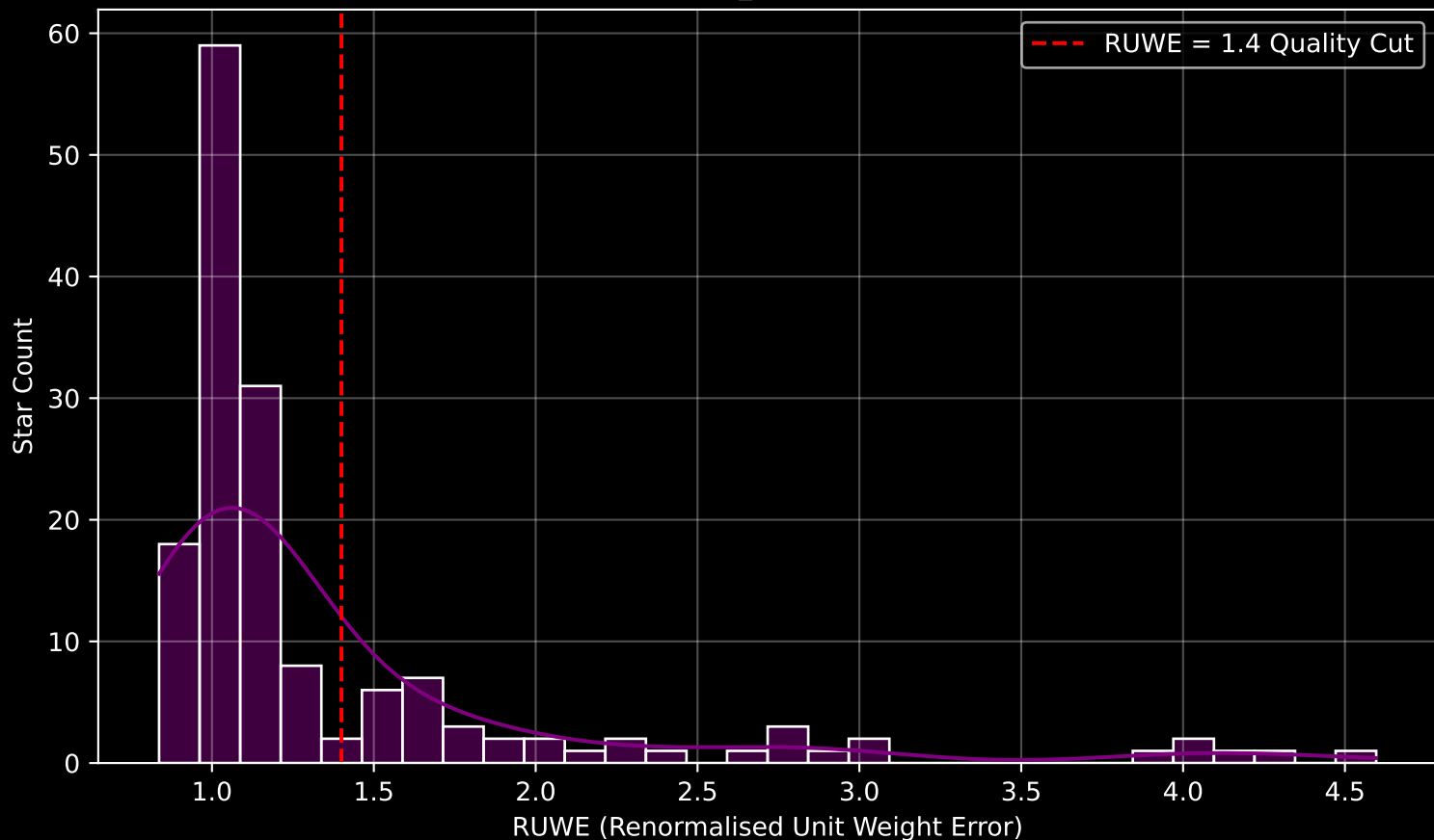
GAPOGEE DR17 Field [041+53_MGA] RUWE Distribution (n= 155)
