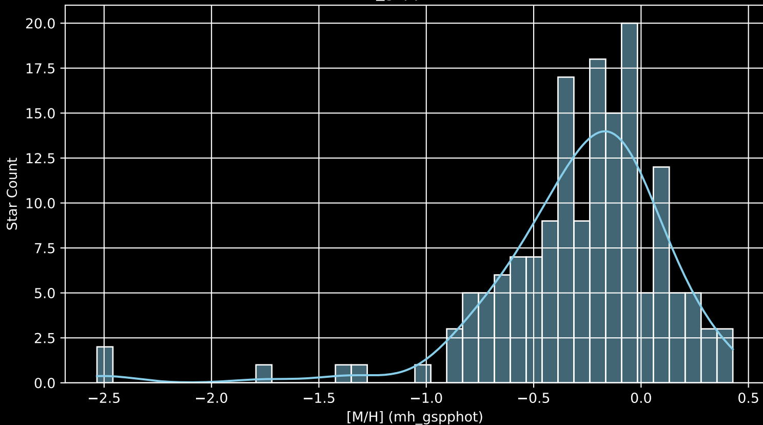
APOGEE DR17 Field: [041+53_MGA [M/H] (mh_gspphot) (n= 160)
