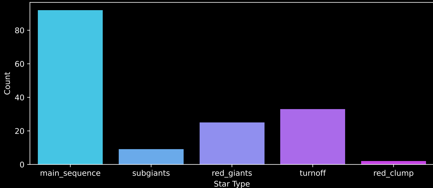
APOGEE DR17 Field: [041+53_MGA] Count plot of Star Type
