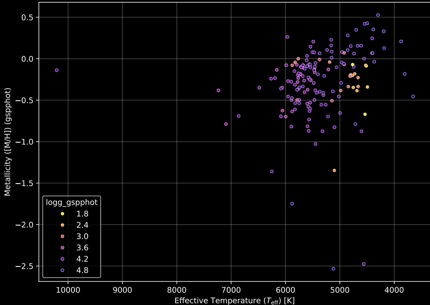
APOGEE DR17 Field: [041+53_MGA] Stellar Population Parameters (n= 161)
